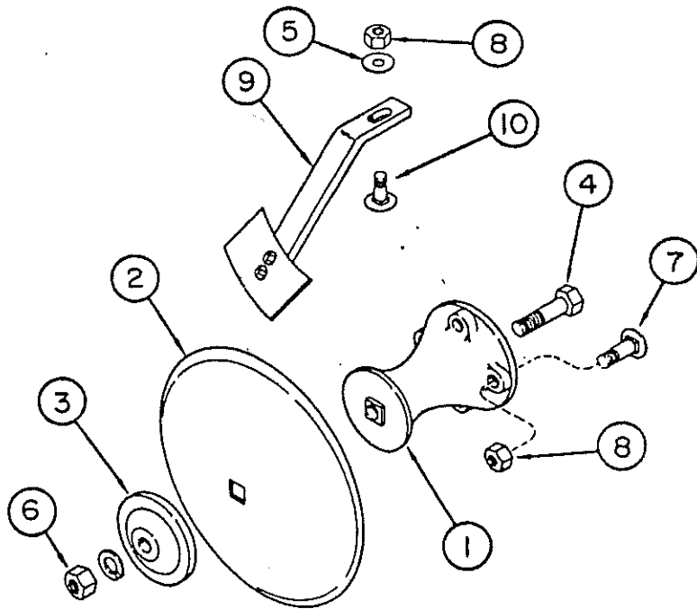
FEATHERING BLADE
