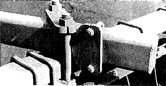
Frame clamps help assure proper frame alignment even under the toughest field conditions.
