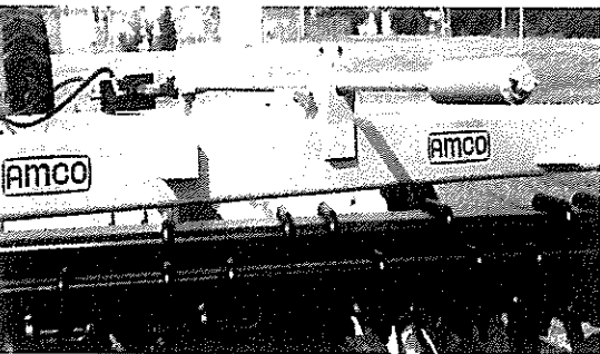
Screw type depth control combined with hydraulic cylinder maintains set cutting depth.
