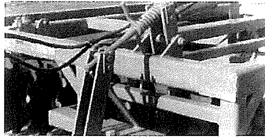
Leveling spring and multiple tongue settings allow adjustments for changes in soil conditions.
