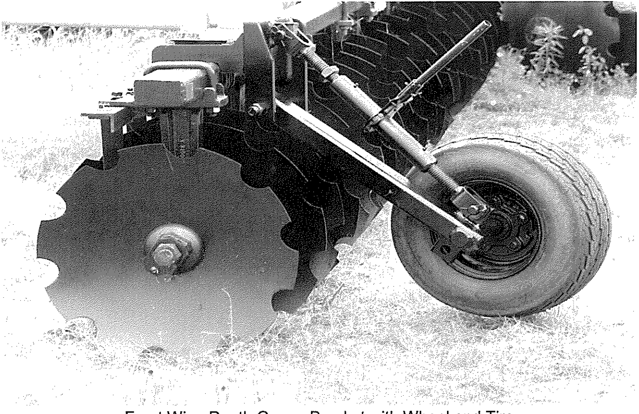
Front Wing Depth Gauge Bracket with Wheel and Tire
