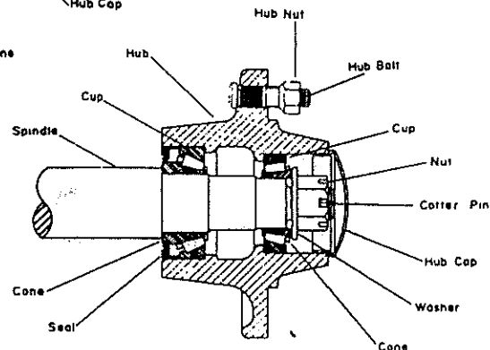
SPINDLE AND HUB FOR WING SECTION
