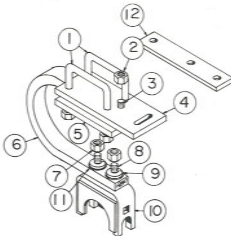
OPTIONAL SHOCK ABSORBER BEARING RISER
