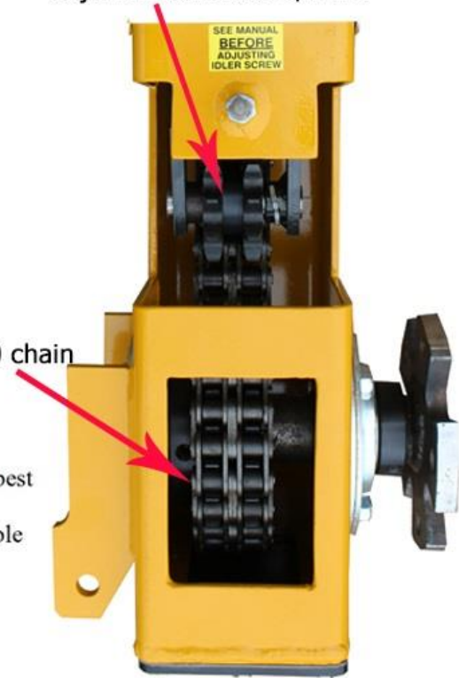
Adjustable steel idler sprocket
