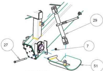
SKID ATTACH SCALE 0.100
