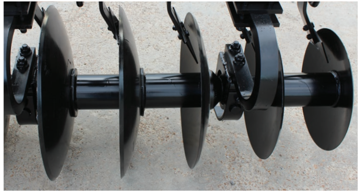
Standard 22" x 1/4" blades (tapered blades on rear gangs).
